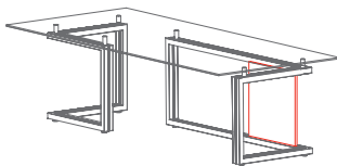
Square modesty panel 1VR1620: L 18 3/4 D 1 H 21 1/4
