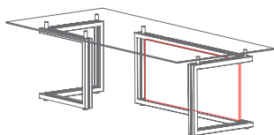
Rectangular modesty panel 1VR1610: L 52 1/4 D 1 H 21 1/4
