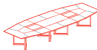
L500 meeting table arranged for electrification, dyed oak solid wood edge and leather top 1VR6511: L 201 D 71 1/4 H 30
