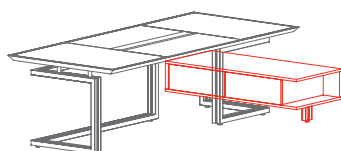
Side container for right desk 1VR2510: L 53 3/8 D 23 1/4 H 10
